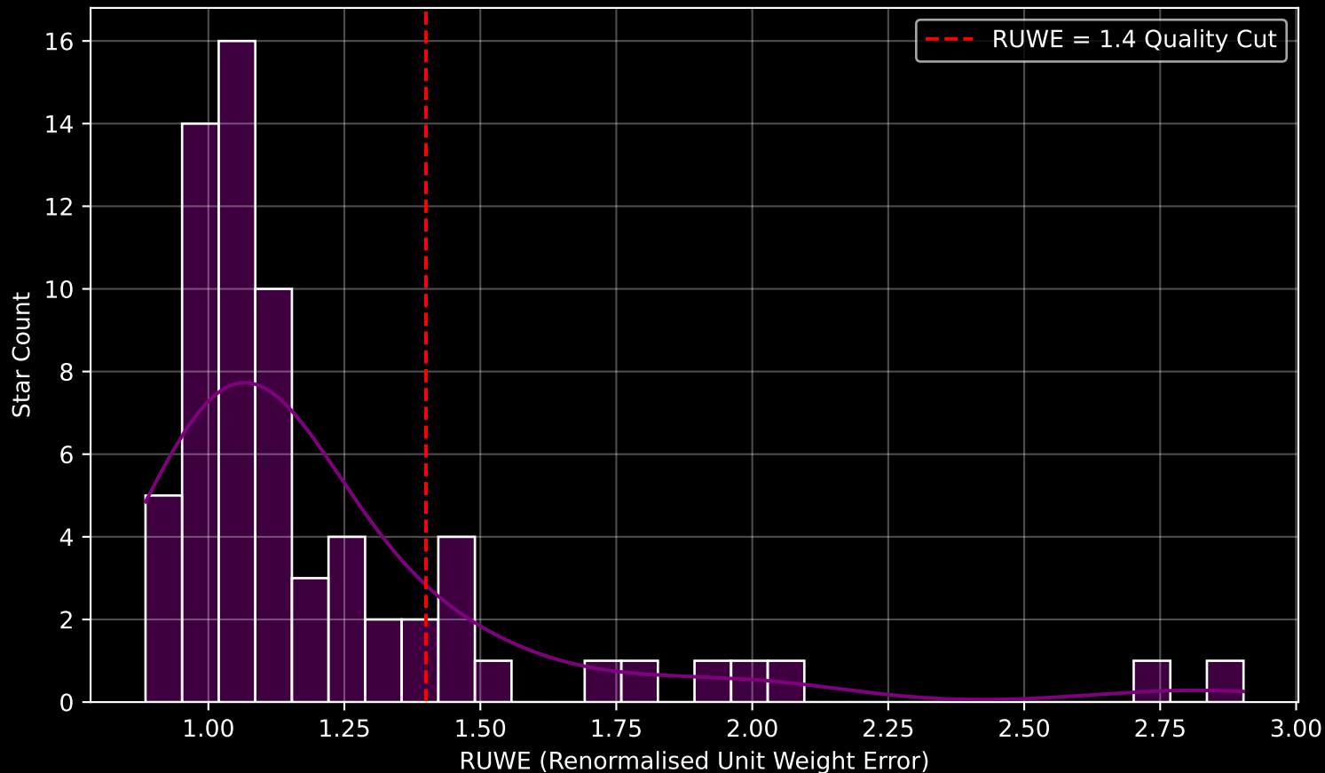
GALAH DR4 Field [6791] RUWE Distribution (n= 68)
