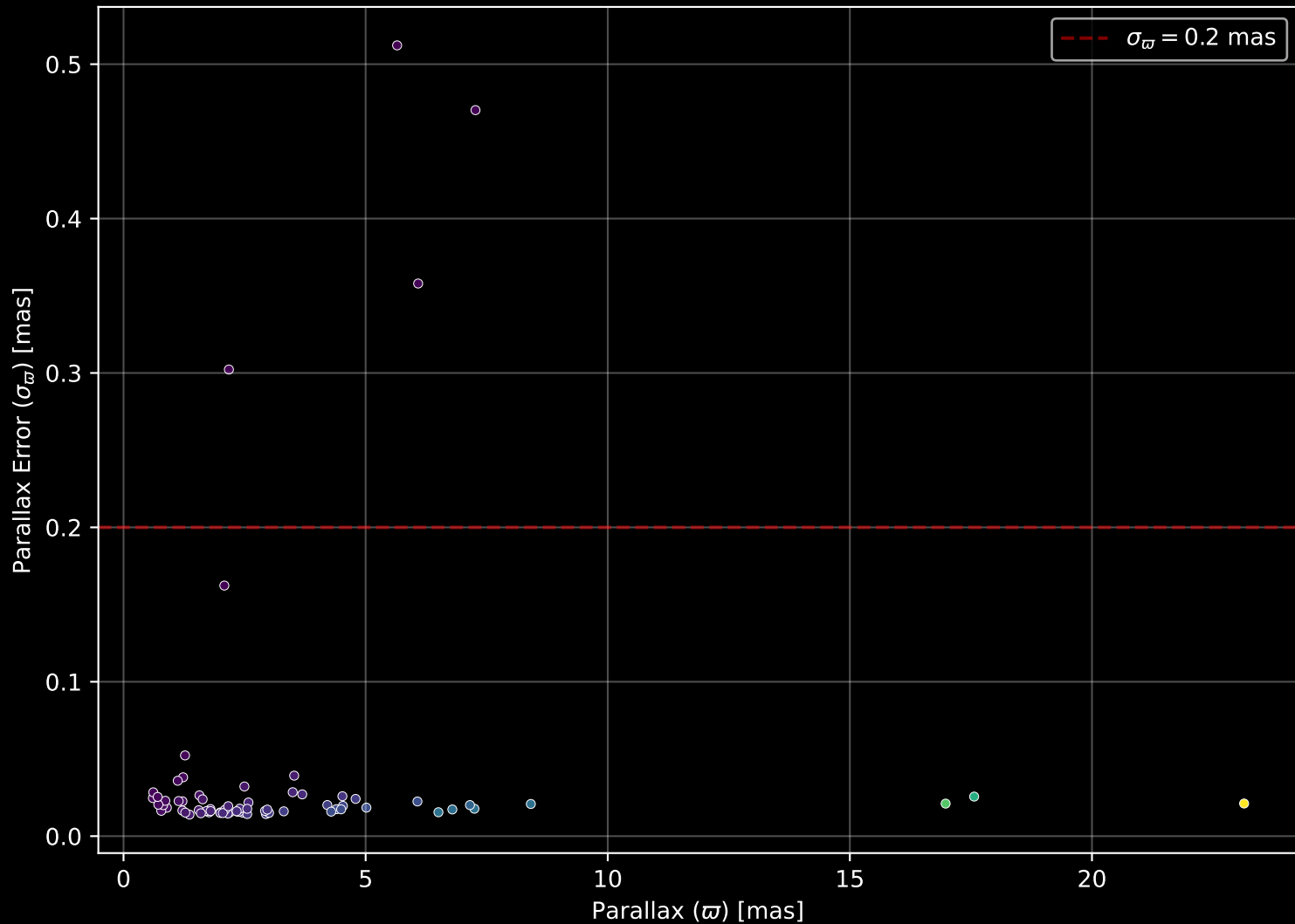
GALAH DR4 Field: [6791] Parallax Quality (n= 73)
