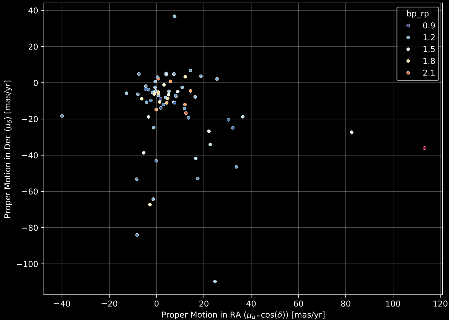
GALAH DR4 Field: [6791] Proper Motion Diagram (n= 73)
