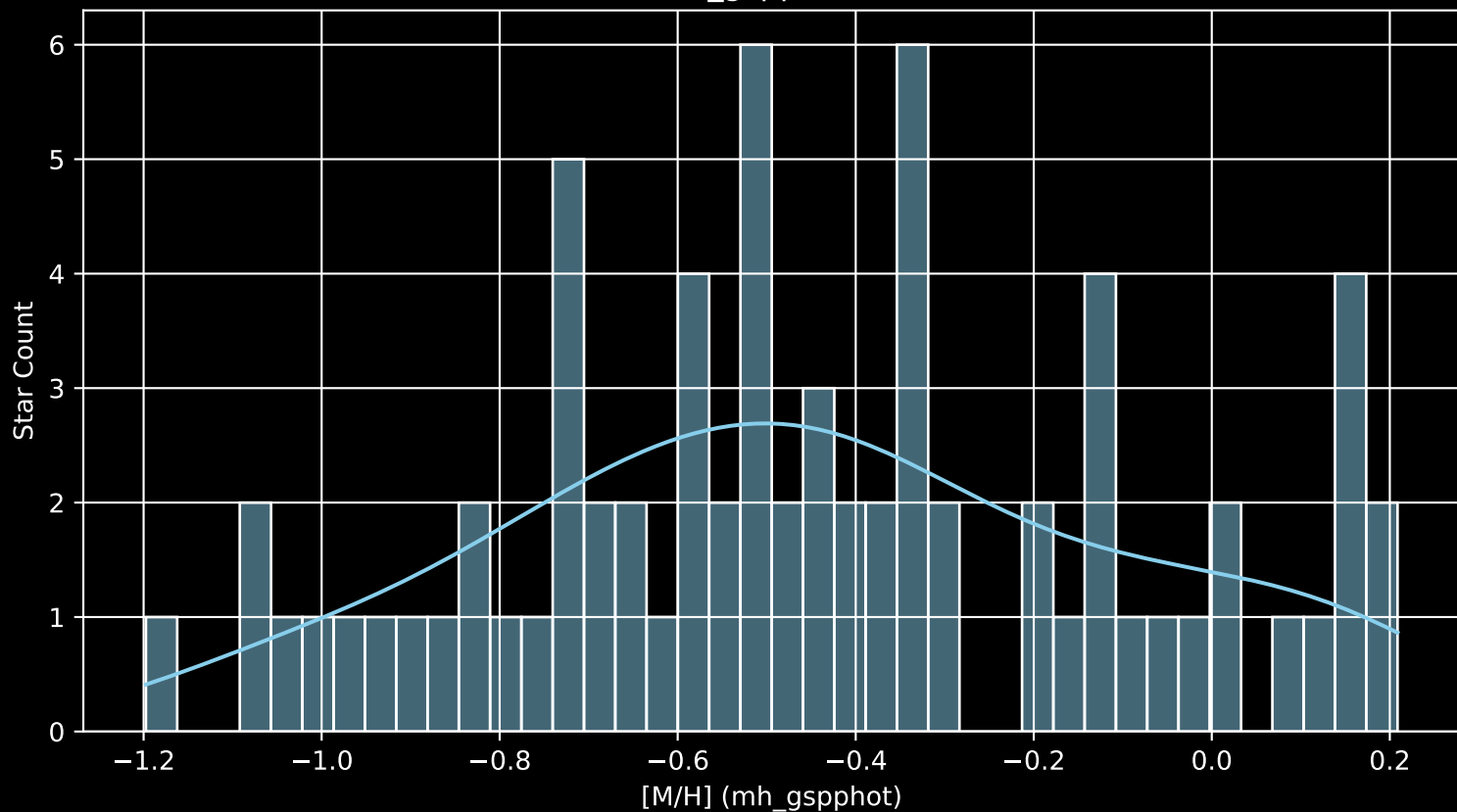
GALAH DR4 Field: [6791] [M/H] (mh_gspphot) (n= 72)
