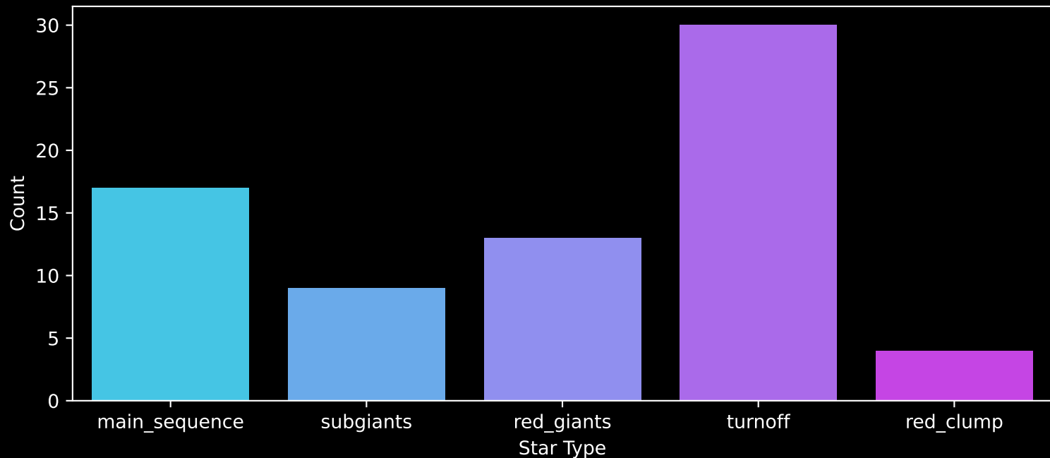
GALAH DR4 Field: [6791] Count plot of Star Type
